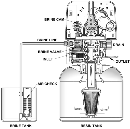
8. Service Position
