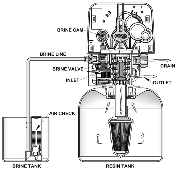
14. Backwash Position
