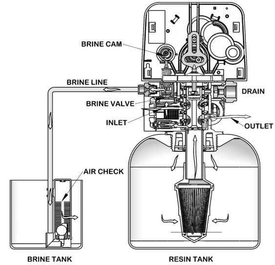
12. Brine Tank Refill Position
