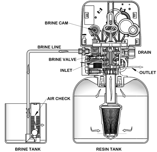
17. Brine Tank Refill Position
