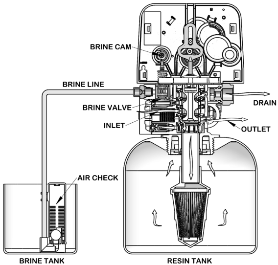
10. Backwash Position
