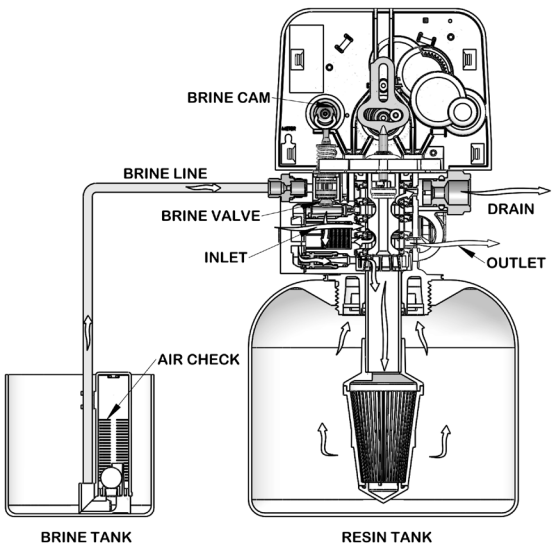
9. Brine/Slow Rinse Position
